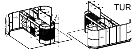
FRONT ISOMETRIC VIEW SCALE: 1/8"
